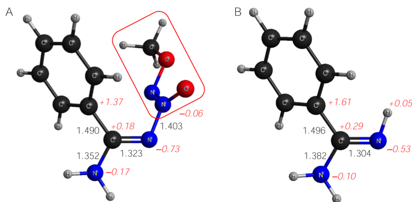
Figure 4. Optimized MP2/ADZ [PCM] structures of 2a (A) and benzamidine (B) together with selected bond lengths (Å) and Mulliken charges (red) where the value of -0.06 corresponds to the O 2 -methylidiazonium diolate group (sum over all of its atoms).
